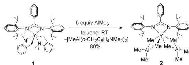
Scheme 2. Synthesis of the heterotrimeric Y/Al complex.
